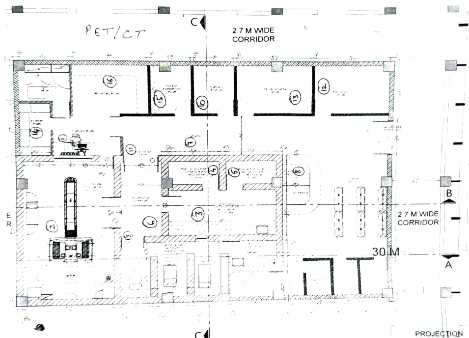
Figure 1: Typical layout and room design of a Nuclear Medicine Department showcasing the segregation of active and non-active zones.
